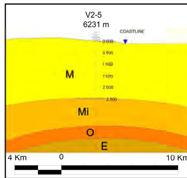
Fig. 18. Sector V2-5 showing a stratigraphic trap at the top of an anticline structure. Vertical scale is in meters. E: Eocene, O: Oligocene, Mi: Lower Miocene, M: Miocene, Q: Quaternary.
