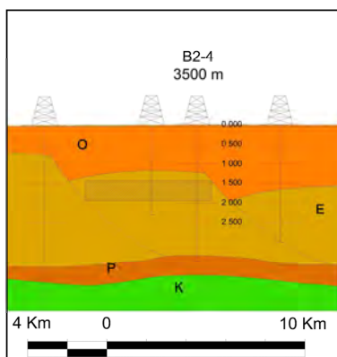
Fig. 10. Sector B2-4 from cross regional section B2. Vertical scale is in meters. K: Cretaceous, P: Paleocene, E: Eocene, O: Oligocene.
