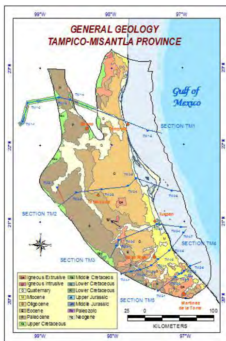
Fig. 12. Simplified geologic map of Tampico-Misantla province displaying regional cross sections and wells. After [33, 34, 35, 37, 46].
