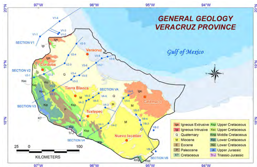
Fig. 16. Simplified geologic map of the Veracruz province, and location of regional geologic sections and wells. After [43, 33, 34, 35, 46].
