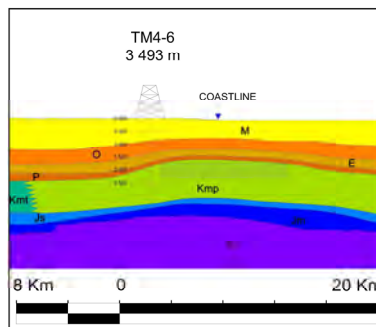
Fig. 14. Sector STM4-6 is overlaying a high basement element. Vertical scale is in meters. Pz: Paleozoic, Jm: Middle Jurassic, Js: Upper Jurassic, Kmt: Middle Cretaceous, Kmp: Middle Cretaceous, P: Paleocene, E: Eocene, O: Oligocene, M: Miocene.
