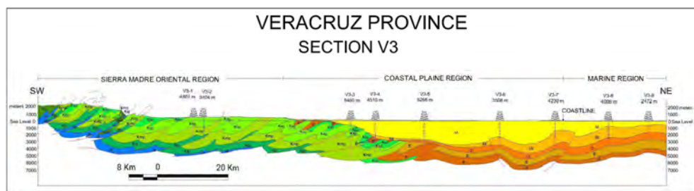
Fig. 17. Regional geological section V3. The left hand side of the regional section shows Zongolica range's Cretaceous carbonate reverse faults as well as the buried tectonic front. The opposite side reveals early Cenozoic deformed terrigenous sequences and late Cenozoic undeformed sedimentary materials. Js: Upper Jurassic, Kip: Lower Cretaceous, Kmp: Middle Cretaceous, Ksp: Upper Cretaceous, Ksc: Upper Cretaceous, P: Paleocene, E: Eocene, O: Oligocene, Mi: Lower Miocene, M: Miocene, Q: Quaternary. After [43, 33, 34, 35, 47].
