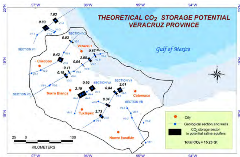
Fig. 19. Sectors with CO 2 storage potential in saline aquifers at the Veracruz province.
