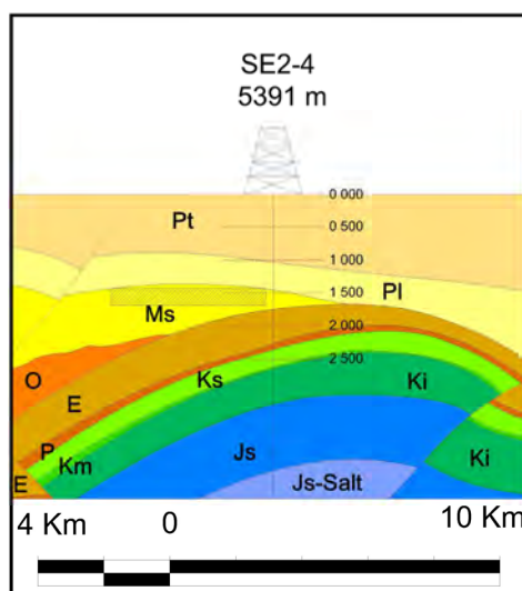
Fig. 22. Sector SE2-4 showing the location of the CO 2 storage target in cross section SE2 of the Sureste province. Vertical scale in meters. Js: Upper Jurassic, Ki: Lower Cretaceous, Km: Middle Cretaceous, Ks: Upper Cretaceous, P: Paleocene, E: Eocene, O: Oligocene, Ms: Upper Miocene, PI: Pliocene, Pt: Pleistocene.
