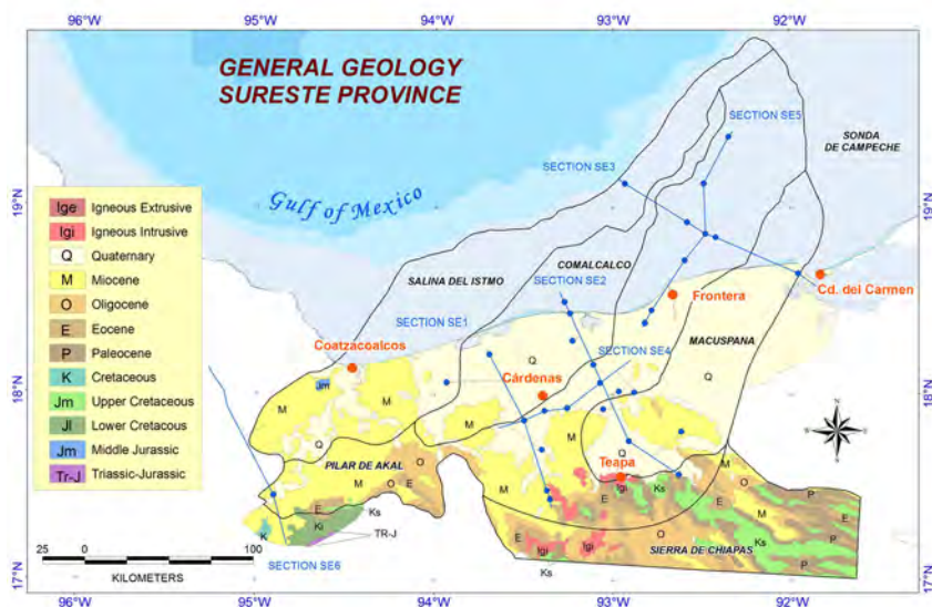
Fig. 20. Simplified geologic map of the Sureste province. It shows the location of regional geologic sections, wells, and limits of subprovinces: Salina del Istmo, Comalcalco, Macuspana and Pilar de Akal. After [33, 34, 35, 41, 44, 45, 46].
