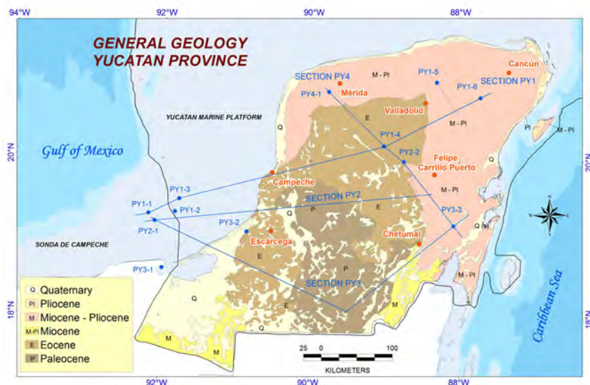
Fig. 24. Simplified geology map of Yucatan province showing regional geologic sections and wells. After [40, 43, 34, 35, 33, 55, 63].
