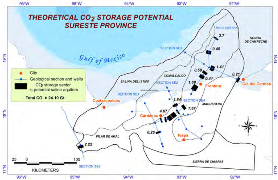
Fig. 23. Sectors shown in black with CO 2 storage potential in saline aquifers at the Sureste province.
