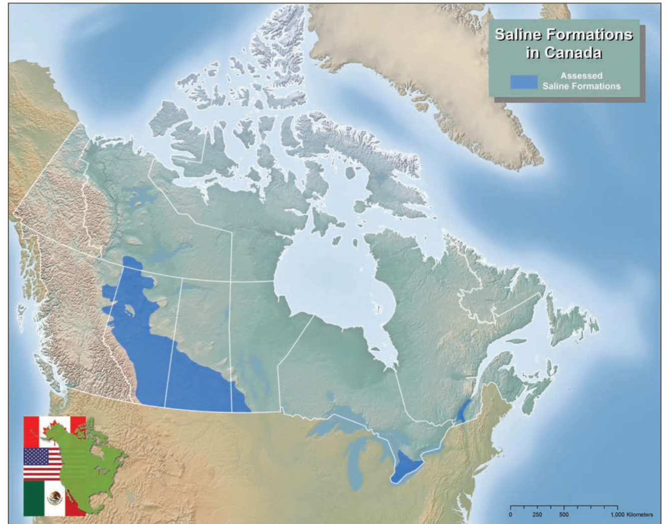
Map shows location of saline formations in Canada assessed in NACSA. Saline formations too far from large CO 2 sources, located in an area of high tectonic activity, located in small intra-montane basins in the Rocky Mountains and in the Atlantic provinces were not evaluated at this time on the basis of a screening process adapted after Bachu (2003). Only the saline formations underlying or close to large stationary sources in Alberta and Saskatchewan in the west (in the Alberta basin and the Canadian portion of the Williston basin) and in central Canada (in the Michigan and Appalachian basins) were evaluated and the results are presented in the table below.
