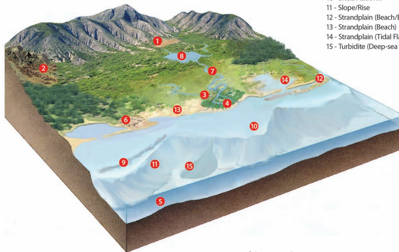
Types of depositional environments.
