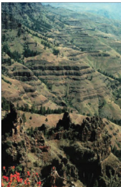
Columbia River Basalt.
